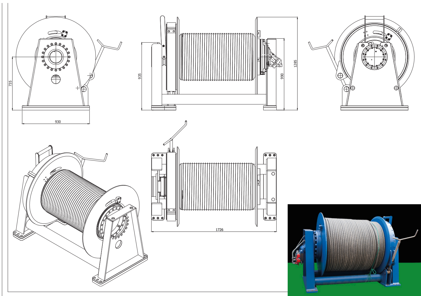
Single drum winch 18 to.
